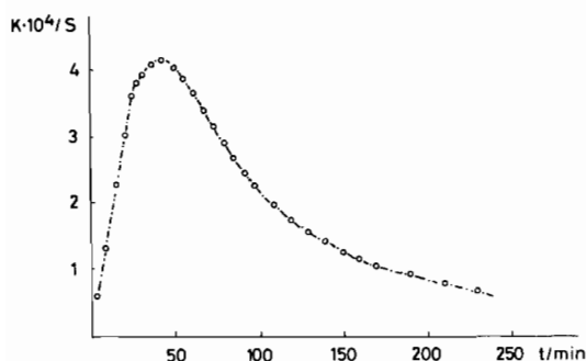
Figure. Conductance vs. time plot for \text{Co(mpt)}_3 + \text{dpae} (mol ratio 1:10; [\text{Co(mpt)}_3] = 1 \times 10^{-3} \text{ mol dm}^{-3} ) in acetone.
